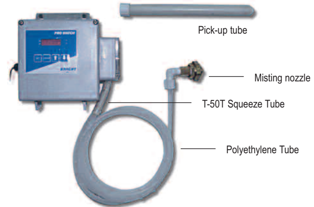
Pro-Watch II 8600385-01
