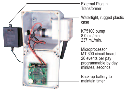
Pro-Watch 510XT
