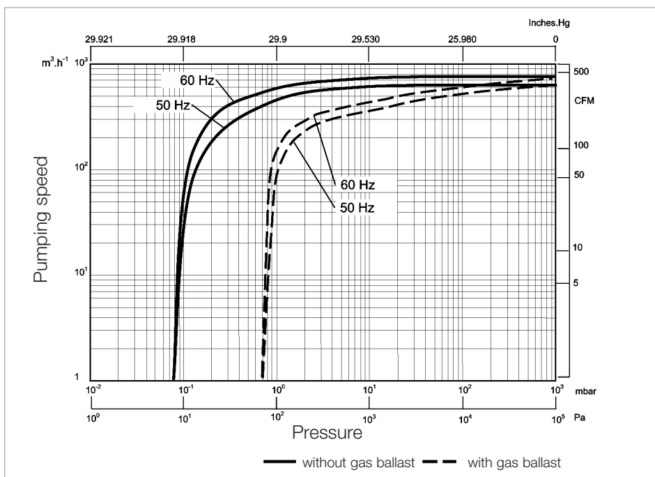
Pumping speed characteristics of the SOGEVAC SV 630 B(F). For SV 750 B(F), refer to the 60 Hz data.
