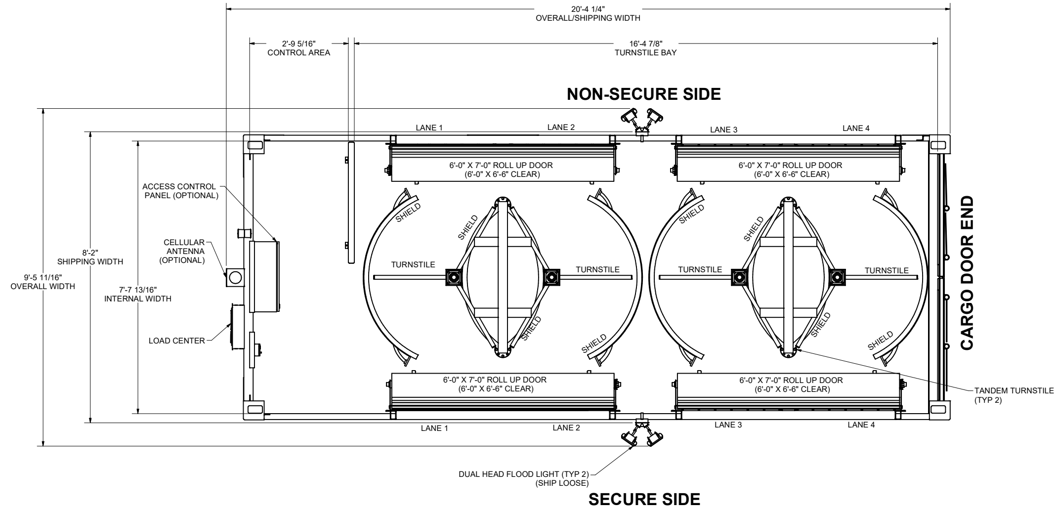
GENERAL ARRANGEMENT - PLAN VIEW SCALE 3/4" = 1'-0"
