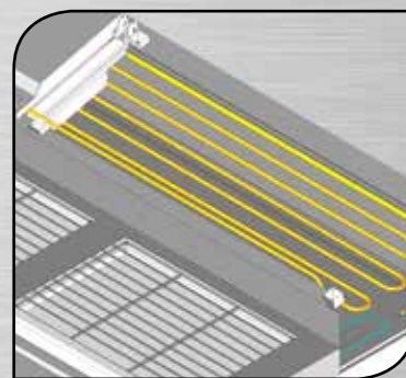
Piping foamed in place (all model 70 / 80)
