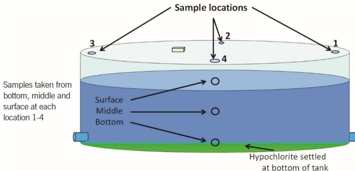
Figure 1. Samples taken from four different areas of the tank (sample locations 1-4) and three different depths within the tank (surface, middle and bottom).
