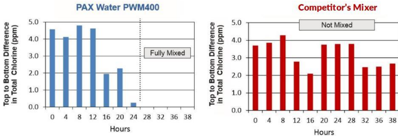
Figure 2. Plots show difference in total chlorine [ppm] between the top and bottom of the tank (averaged across all four sample sites). The PWM 400 achieved mixing in 24 hours. The competitor's mixer failed to mix the tank.
