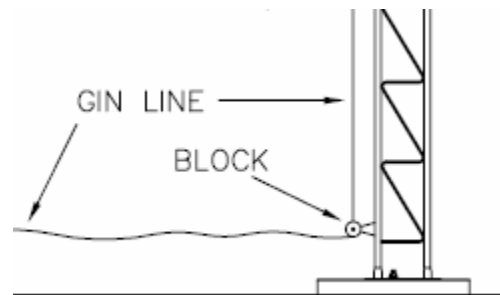
Snatch Block in use at ground level
