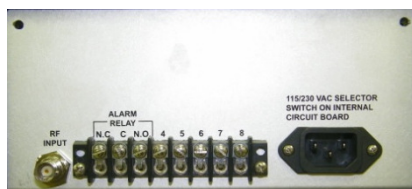
Rear View of MR-5 Rack Mount
