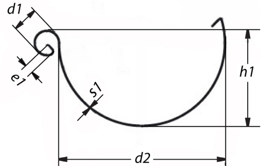
Gutter-cross-section
